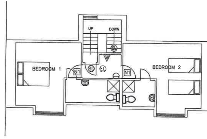
ATTIC FLOOR PLAN 1/100
